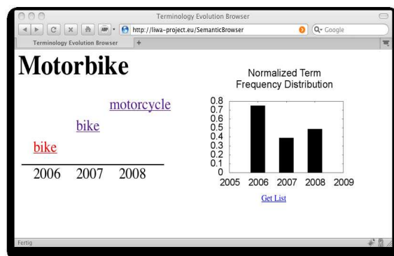
Figure 5: User-interface showing clusters for term Motorbike
