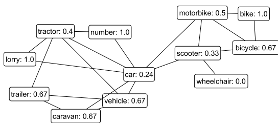
Figure 4: Subgraph from .gov.uk archive from 2006, each node contains also its clustering coefficient from the local graph. The graph shows two clusters which both correspond to means of transportation.
