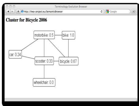
Figure 6: Graphical representation of 2006's Motorbike-Cluster
